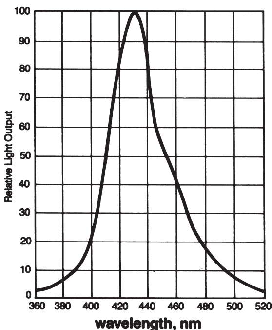
Emission Spectrum
